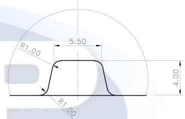
SPOT BAR DETAIL A (5 : 1)
