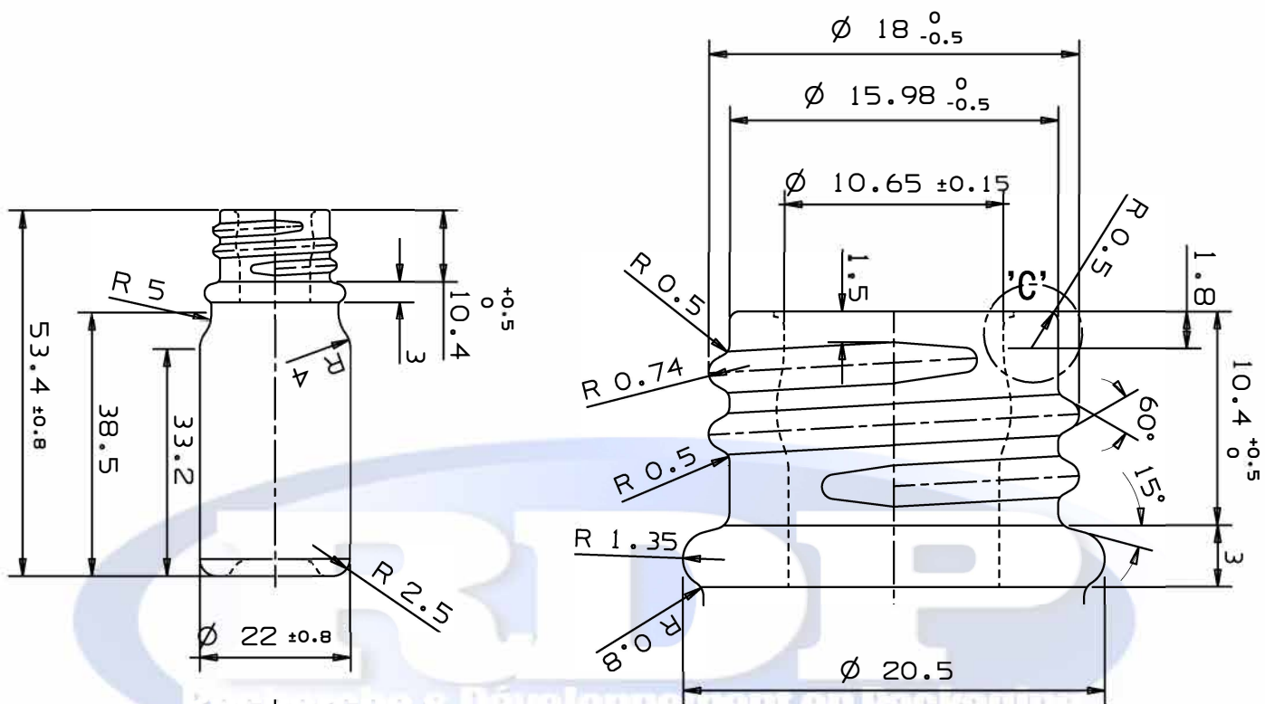
FINISH DETAILS SCALE 3:1
