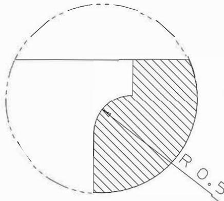
DETAIL C 20:1
