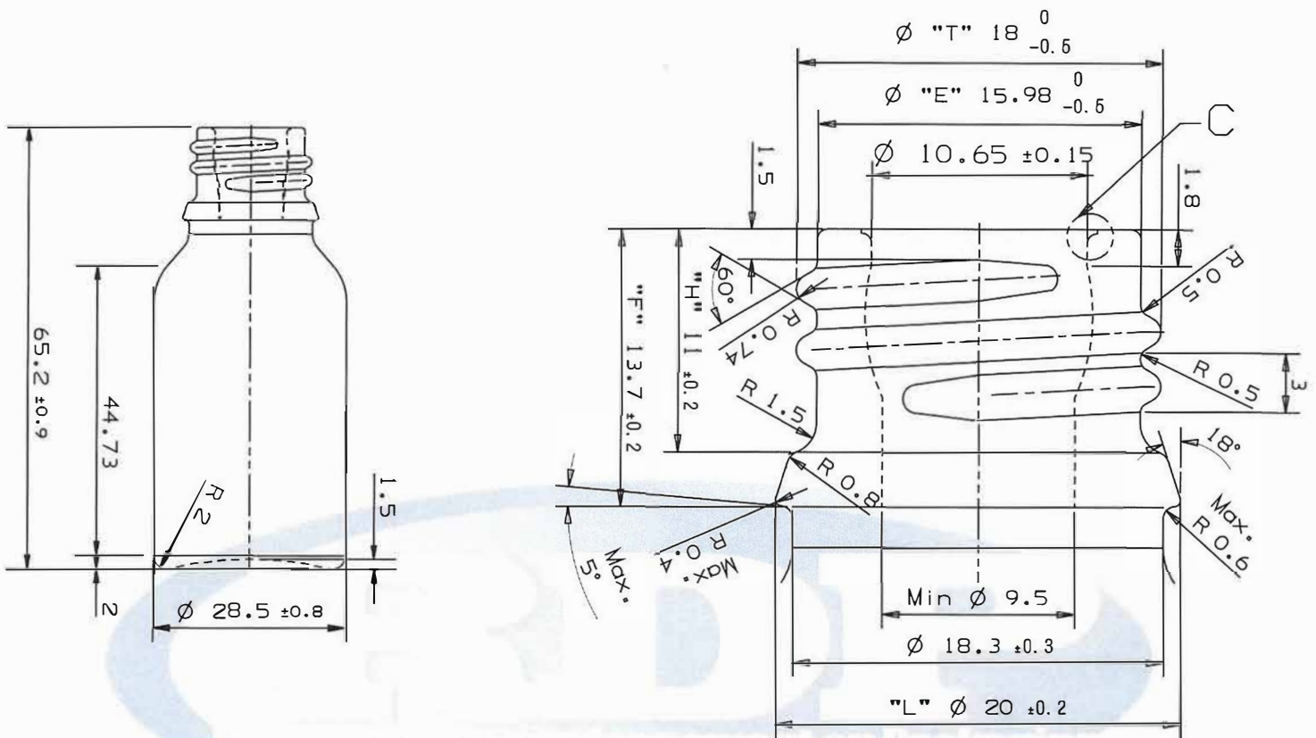
FINISH DETAILS SCALE 3:1
